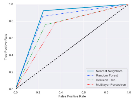
(b) The comparison of classifier ROC curves.
