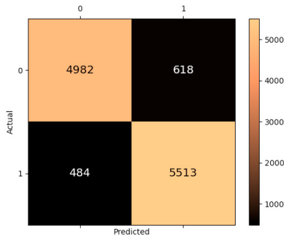
(a) The confusion matrix of the best ranked KNeighbors classifier.
